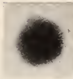
Strain VTS.
